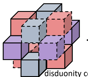
Cluster of Cubes
