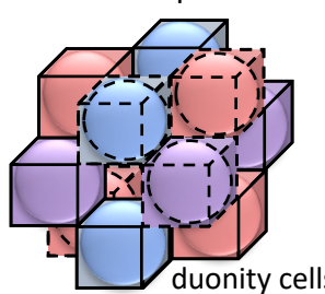
Cluster of SphereCubes
