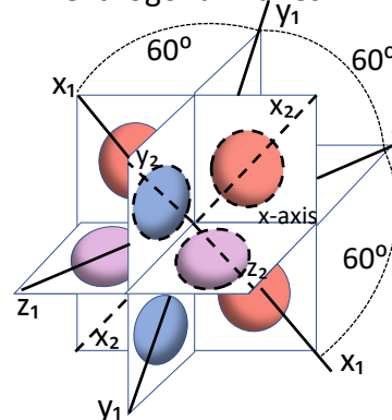
Cluster of SphereCubes
