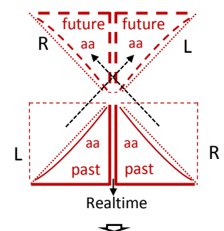
Spacetime Lightcone
